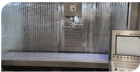
3-axis DMG DMF 220 Linear. XYZ 2200 x 560 x 720 mm, SK40, CTS
